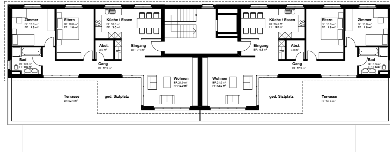
Attikageschoss
